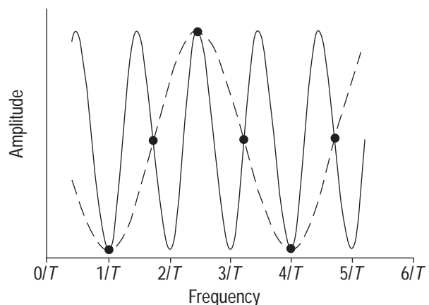
Fig. 1. - Aliasing. If a sine wave of frequency 1/T (—) is sampled at a rate of 4/3T (●), samples of a sine wave of frequency 1/3T (---) are obtained.
